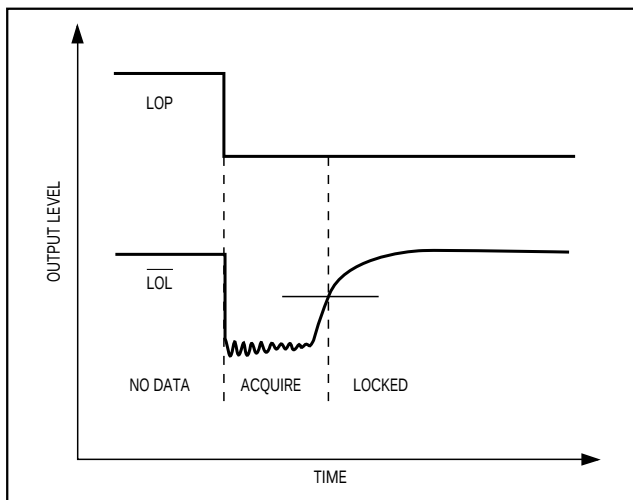
Figure 4. Loss-of-Lock Output
