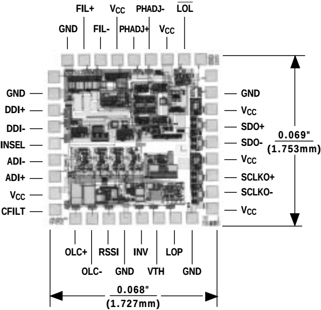
Chip Topography
