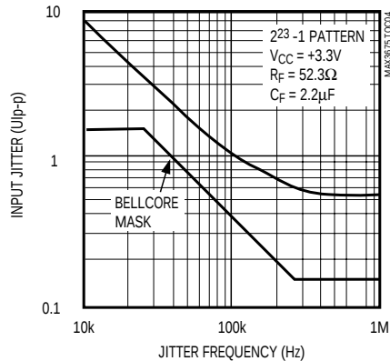
JITTER TOLERANCE
