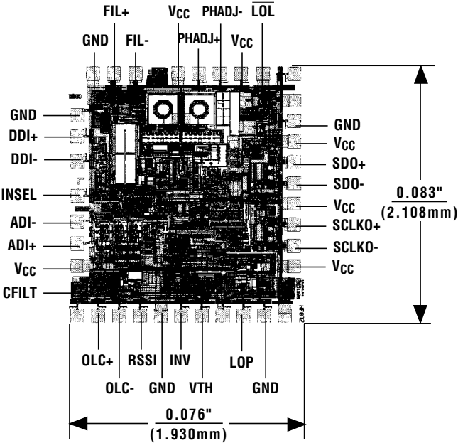
Chip Topography
