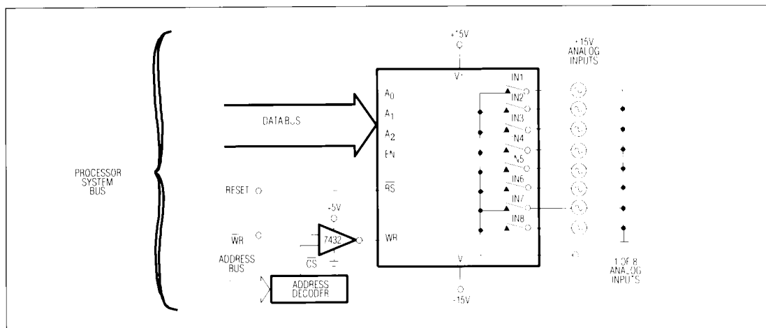
Figure 13. Bus Interface
