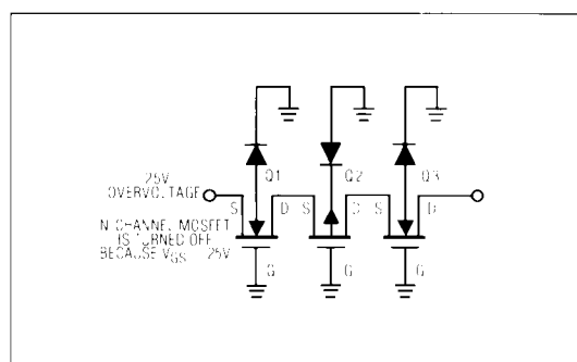
Figure 9. +25\text{V} Overvoltage with Multiplexer Power OFF
