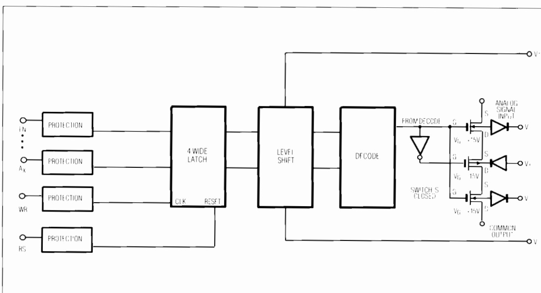
Figure 12. Simplified Internal Structure
