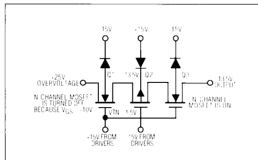
Figure 11. +25\text{V} Overvoltage Input to the ON Channel
