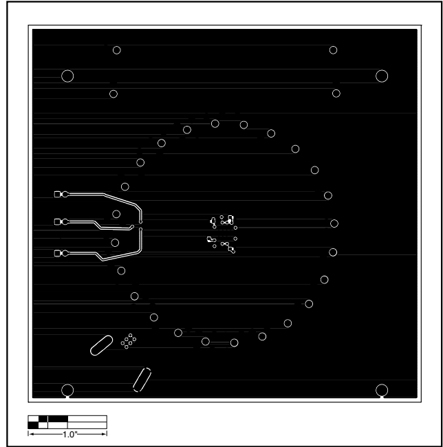
Figure 4. MAX3781 EV Kit PC Board Layout—Solder Side
