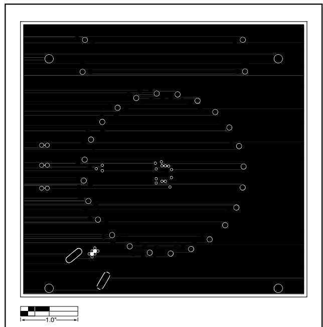
Figure 6. MAX3781 EV Kit PC Board Layout—Ground Plane
