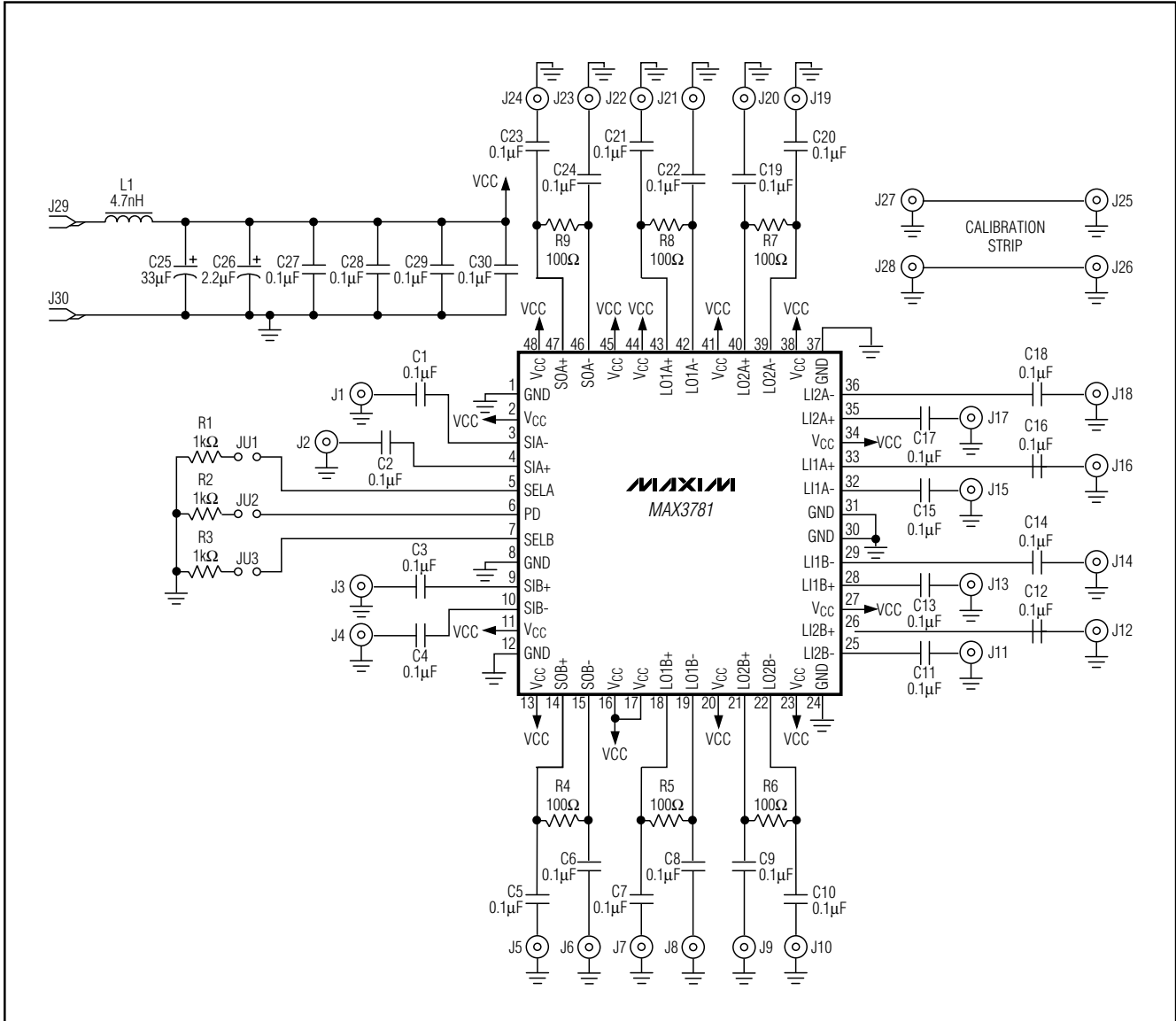
Figure 1. MAX3781 EV Kit Schematic
