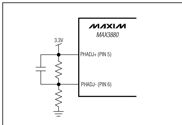
Figure 6. Phase-Adjust Resistor-Divider
