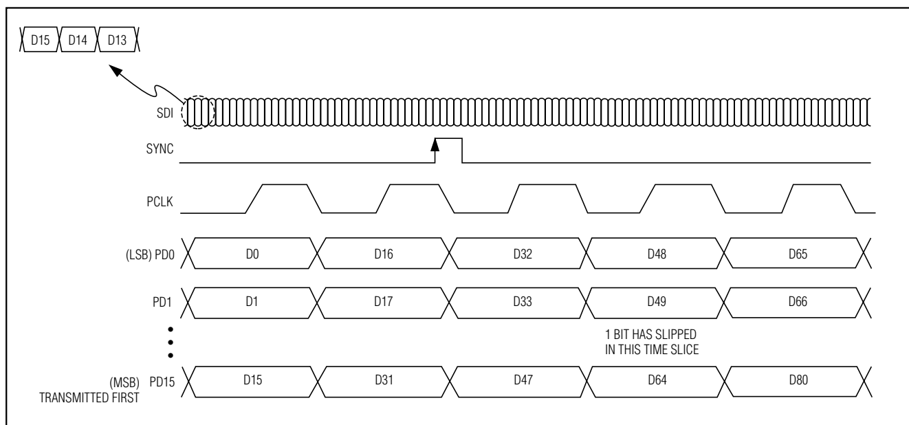
Figure 4. Timing Diagram
