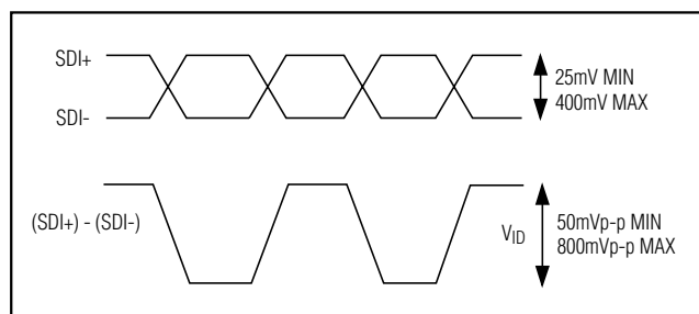
Figure 1. Input Amplitude
