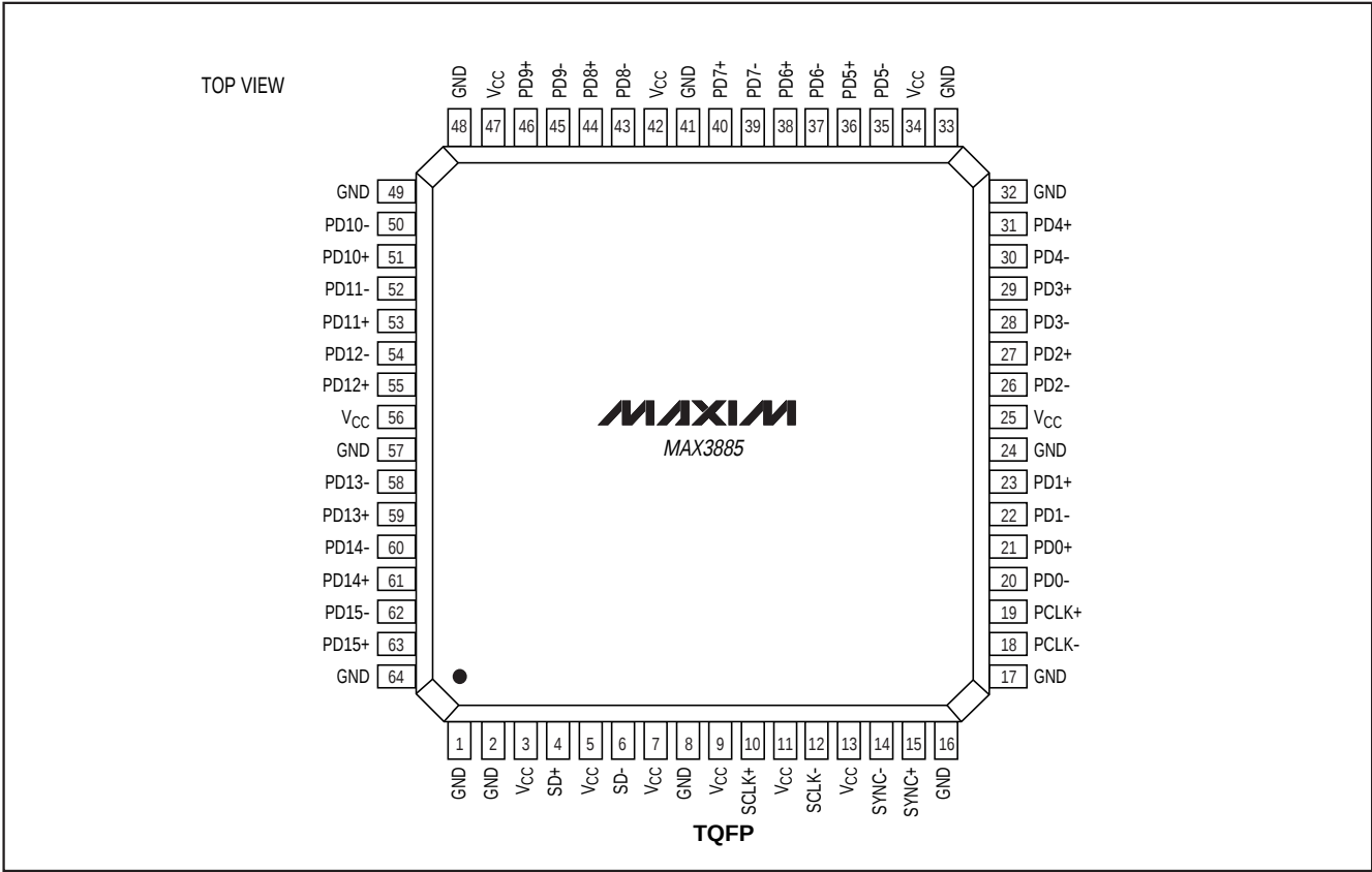
Pin Configuration
