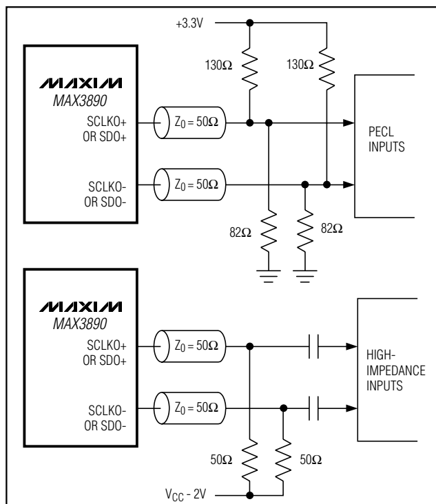
Figure 4. Alternative PECL-Output Termination
