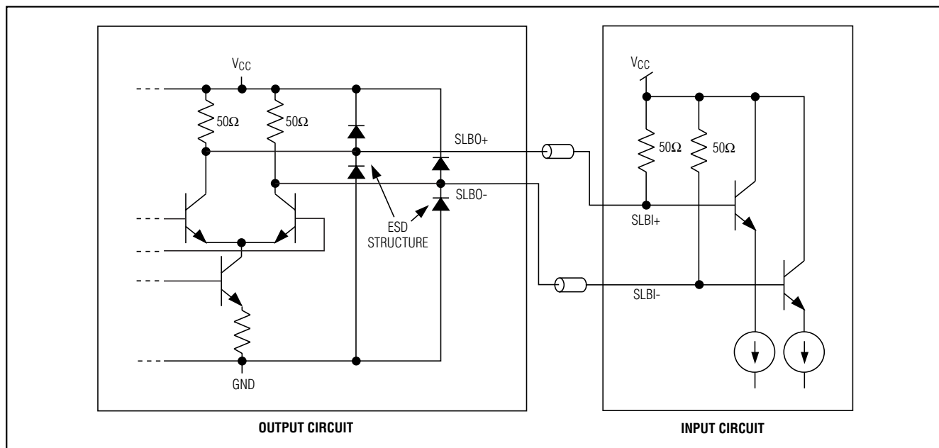
Figure 3. Current-Mode Logic
