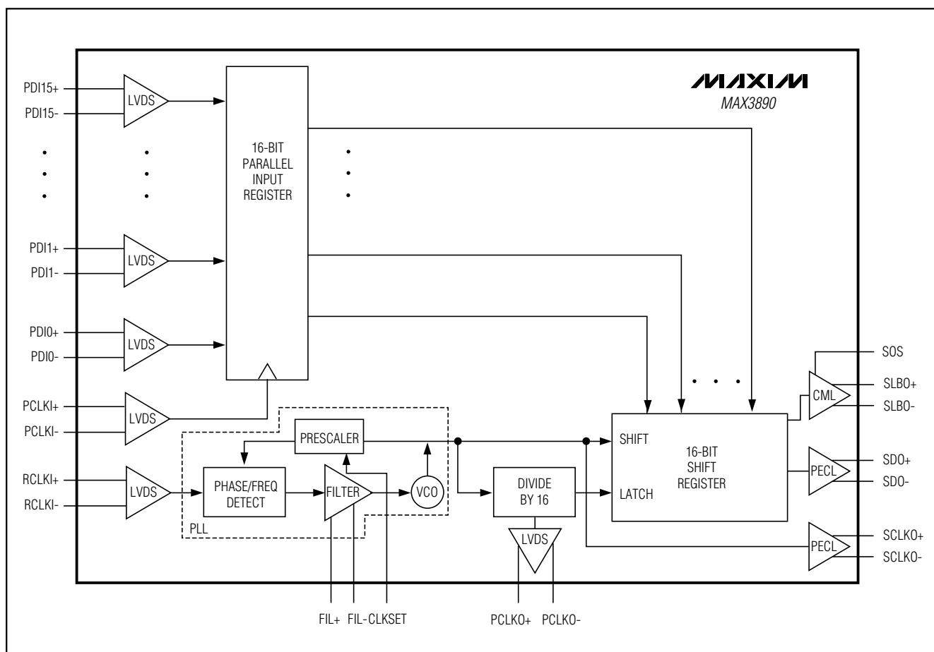
Figure 1. Functional Diagram
