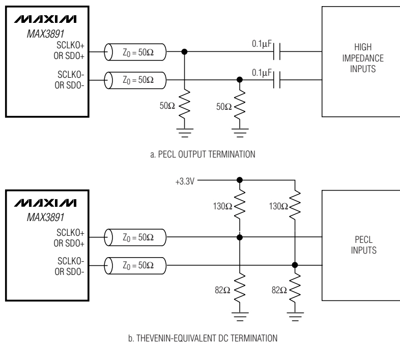
Figure 4. Alternative PECL-Output Termination
