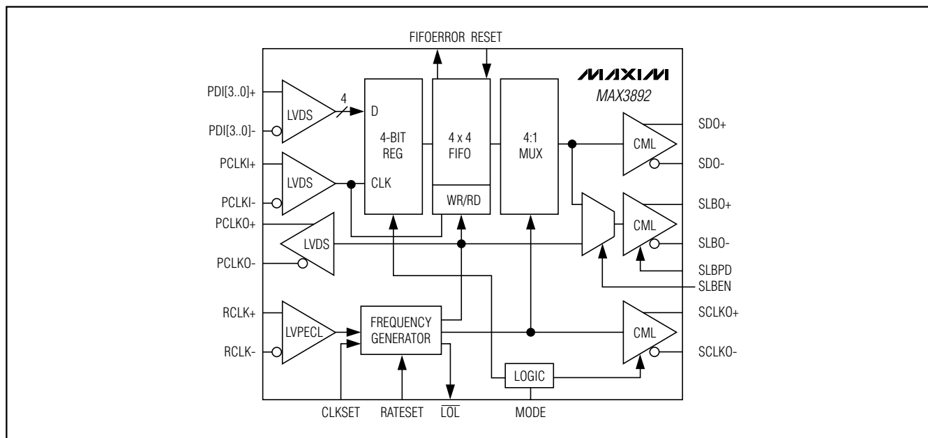
Figure 2. Functional Diagram
