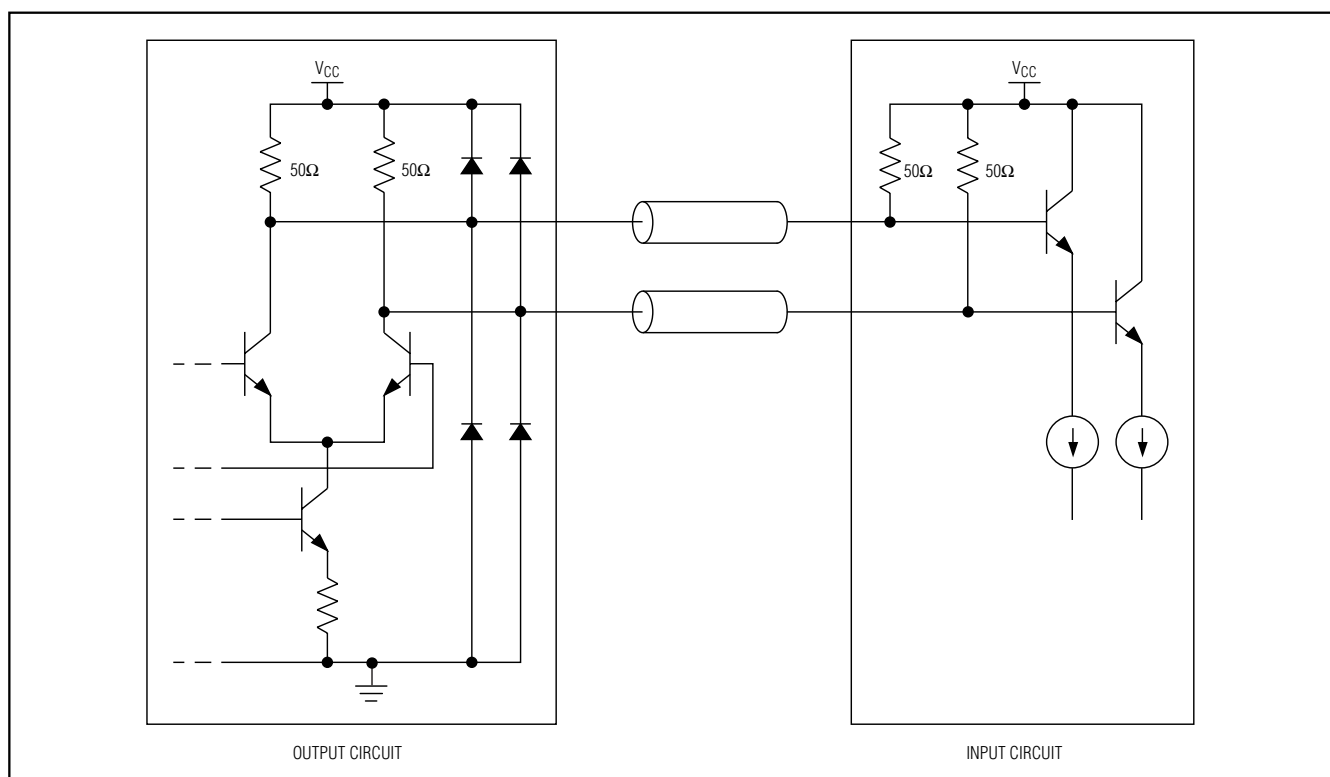
Figure 3. Current-Mode Logic
