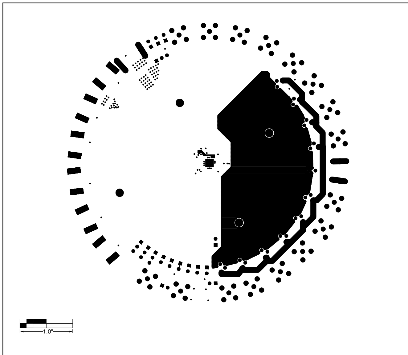
Figure 7. MAX3892 EV Kit PC Board Layout—Solder Side
