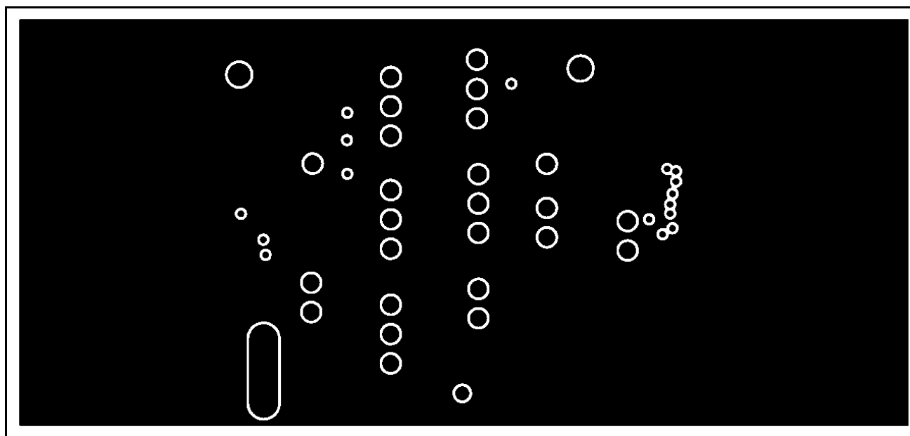
Figure 3. MAX3940 EV Kit PC Board Layout—Ground Plane
