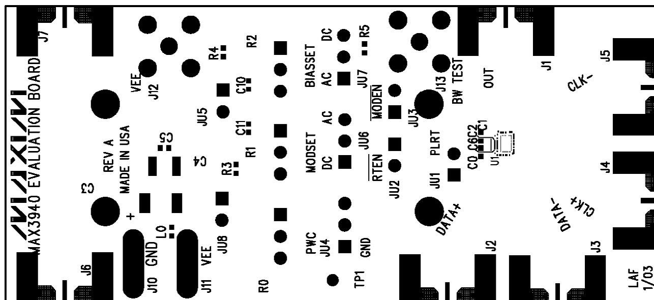
Figure 2. MAX3940 EV Kit Component Placement Guide—Component Side
