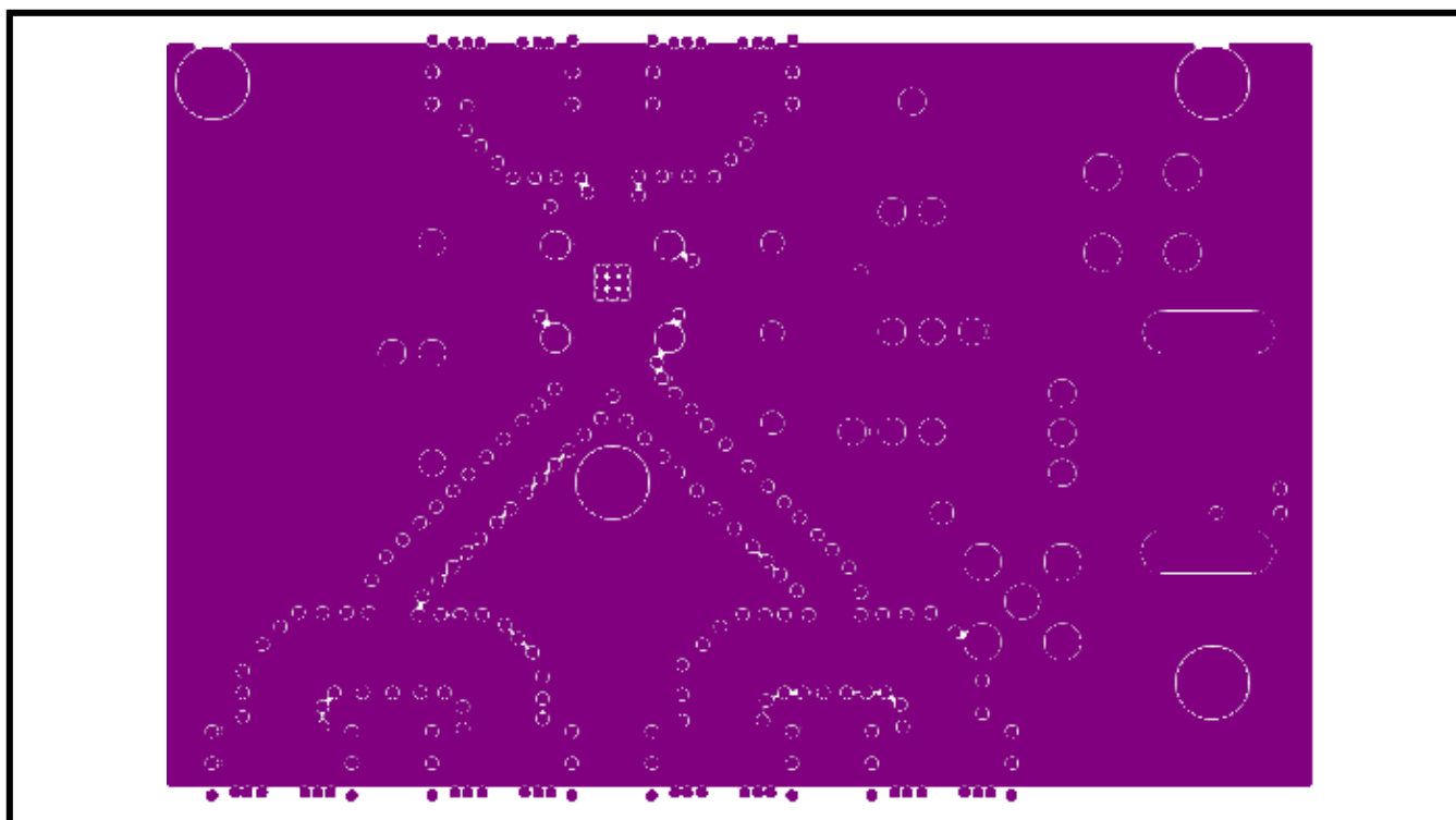
Figure 5. MAX3942 EV Kit PC Board Layout—Power Plane
