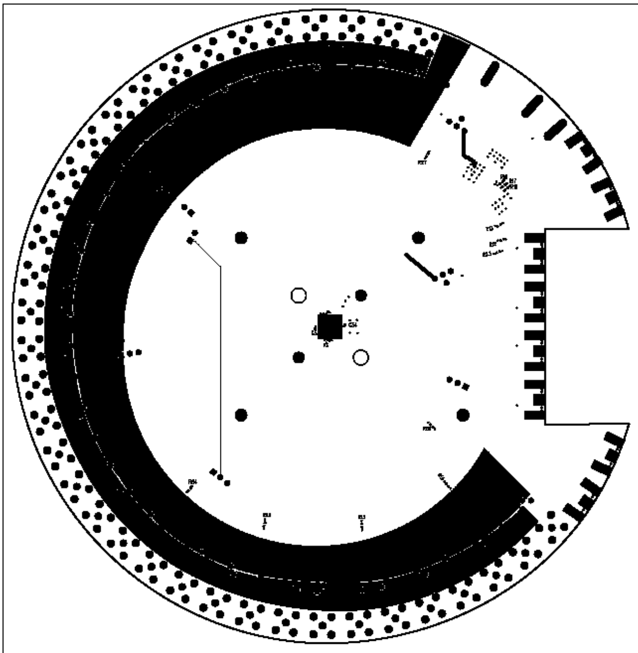
Figure 6. MAX3952 EV Kit PC Board Layout—Solder Side
