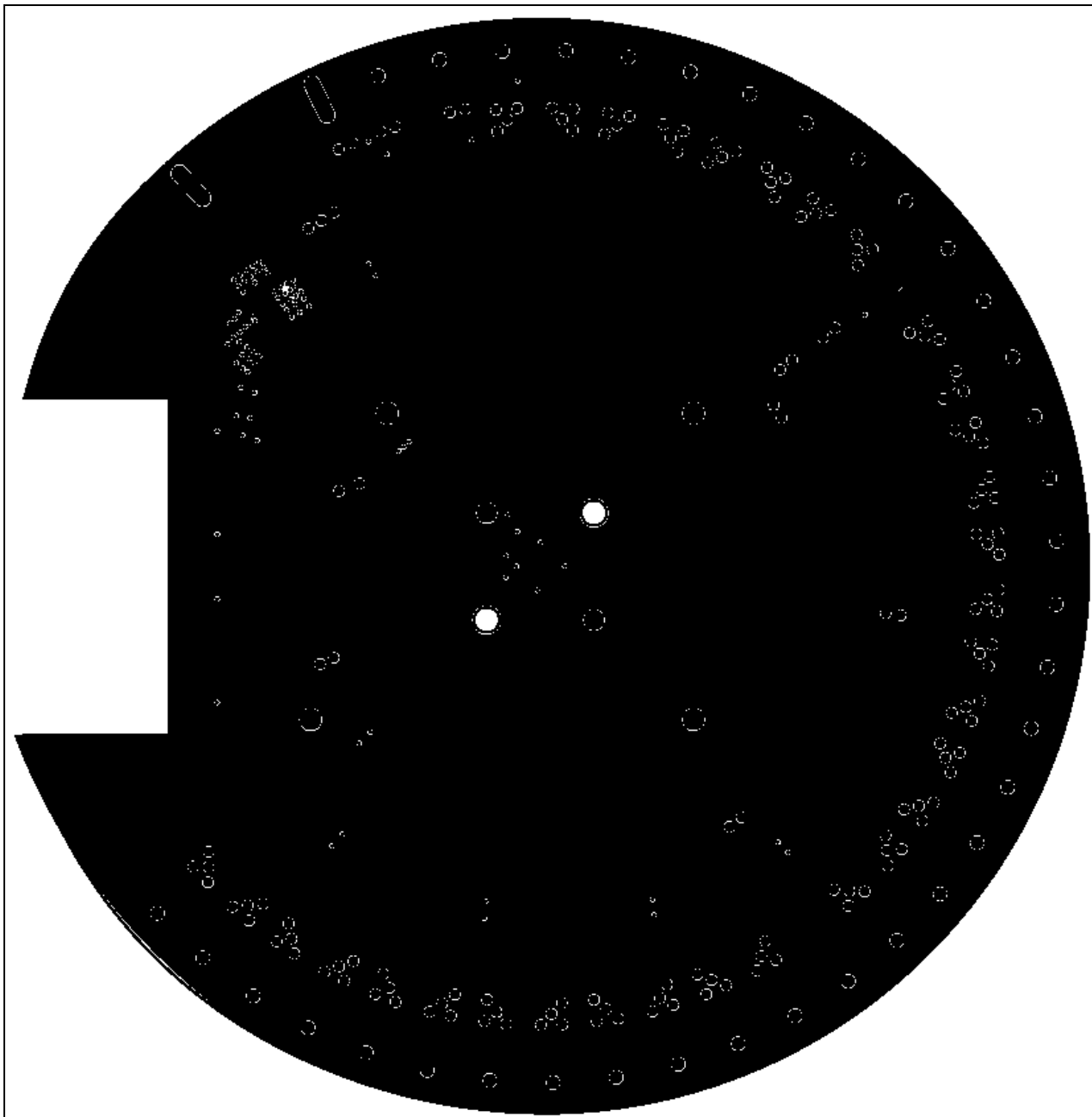
Figure 8. MAX3952 EV Kit PC Board Layout—Ground Plane
