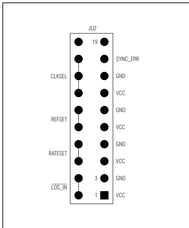
Figure 1. JU2 Header Configuration
