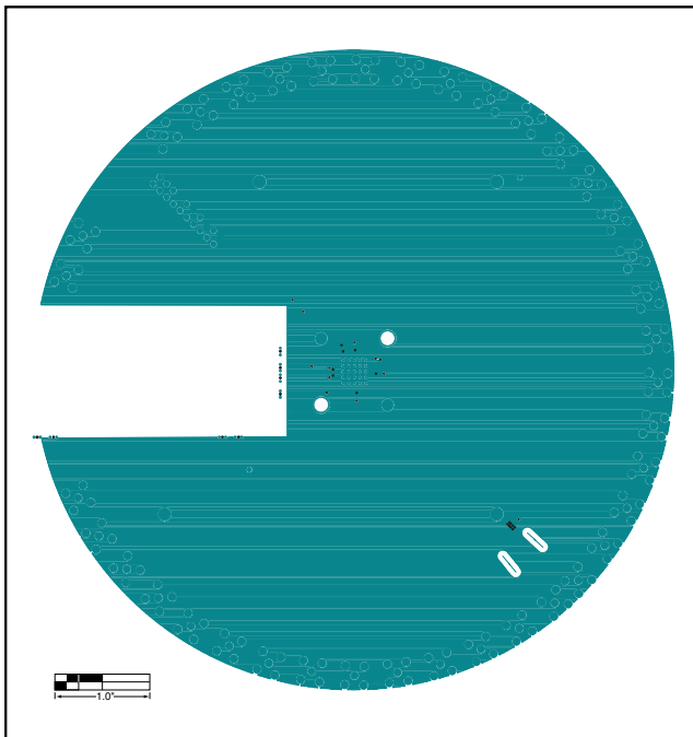
Figure 6. MAX3953 EV Kit PC Board Layout—Power Plane
