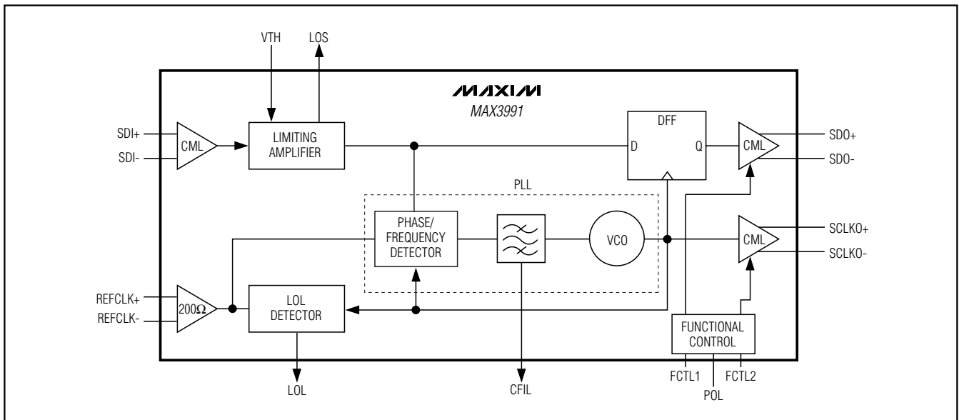
Figure 3. Functional Diagram
