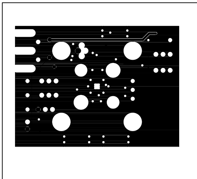
Figure 6. MAX3996 EV Kit PC Board Layout—Power Plane
