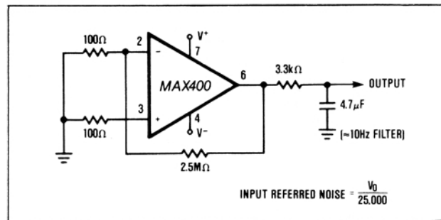
Figure 2. Low Frequency Noise Test Circuit.
