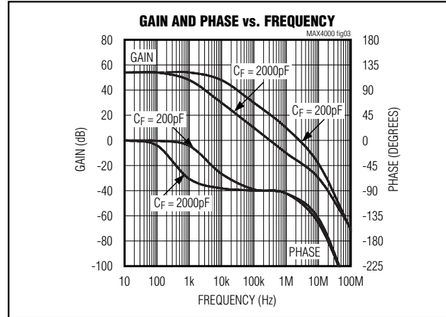
Figure 3. Gain and Phase vs. Frequency Graph
