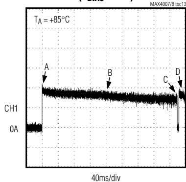
SHORT-CIRCUIT RESPONSE ( V_{\text{BIAS}} = 76\text{V} )
