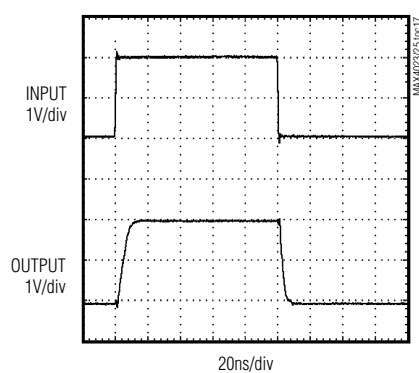
MAX4023/MAX4025 LARGE-SIGNAL TRANSIENT RESPONSE
