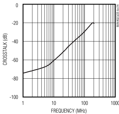
ALL-HOSTILE CROSSTALK vs. FREQUENCY
