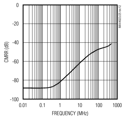
MAX4023/MAX4025 COMMON-MODE REJECTION RATIO vs. FREQUENCY
