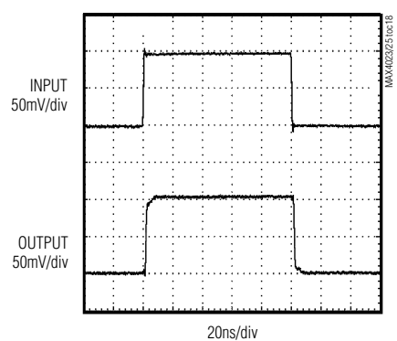
MAX4023/MAX4025 SMALL-SIGNAL TRANSIENT RESPONSE
