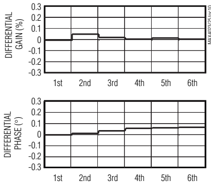
MAX4024/MAX4026 DIFFERENTIAL GAIN AND PHASE
