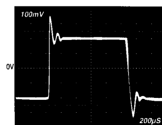
MAX409/MAX417/MAX419 SMALL-SIGNAL TRANSIENT RESPONSE
