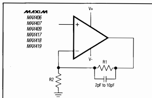
Figure 2. Compensation for Feedback Node Capacitance
