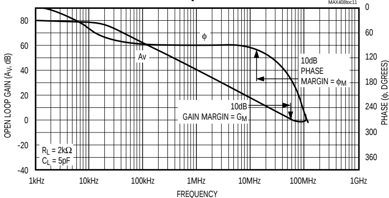
OPEN LOOP FREQUENCY RESPONSE
