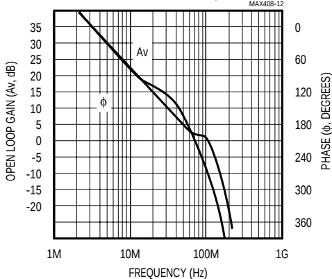
OPEN LOOP FREQUENCY RESPONSE, R_L = 50\Omega , C_L = 50\text{pF}
