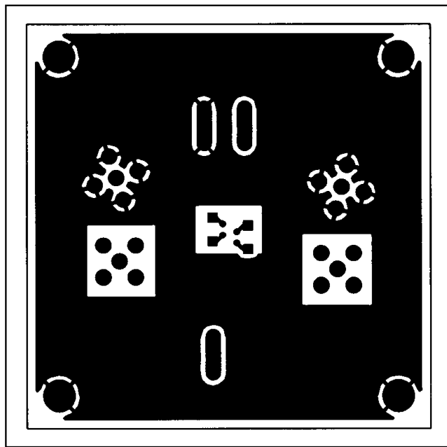
Figure 6. PC Board Layout—Solder Side
