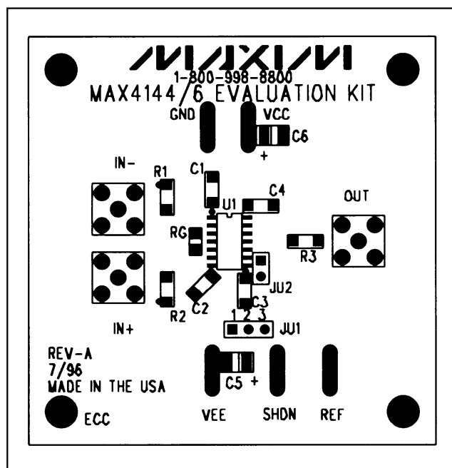
Figure 2. MAX4144 EV Kit Component Placement Guide— Component Side
