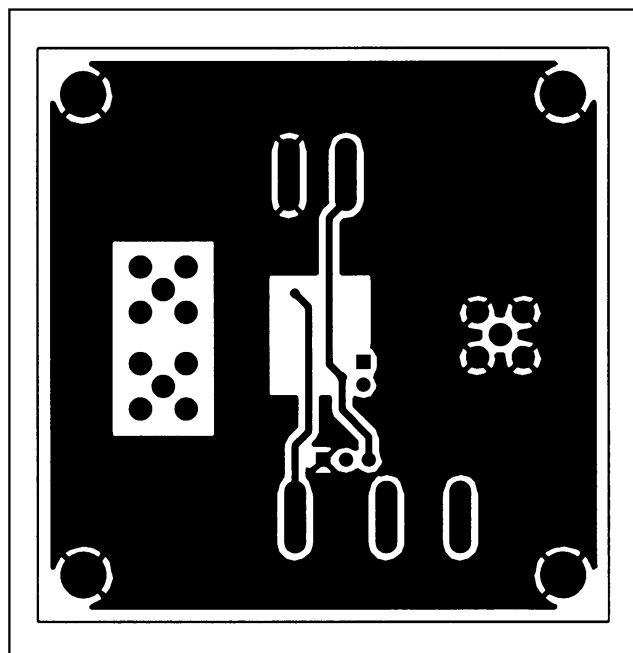
Figure 4. MAX4144 EV Kit PC Board Layout—Solder Side
