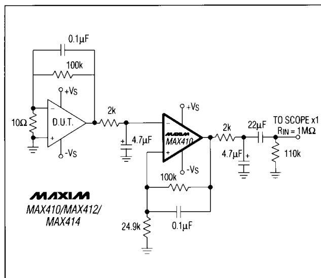
Figure 3. 0.1Hz to 10Hz Voltage Noise Test Circuit
