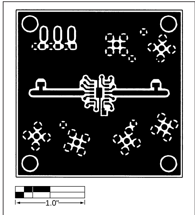
Figure 3. MAX4188 EV Kit PC Board Layout—Component Side
