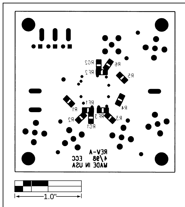
Figure 5. MAX4188 EV Kit Component Placement Guide—Solder Side
