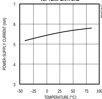
POWER-SUPPLY CURRENT (PER AMPLIFIER) vs. TEMPERATURE
