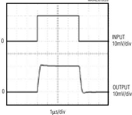
MAX4236 NONINVERTING SMALL-SIGNAL RESPONSE MAX4236 toc28
