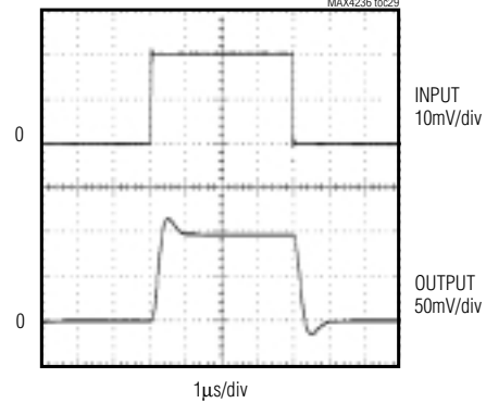
MAX4237 NONINVERTING SMALL-SIGNAL RESPONSE MAX4236 toc29
