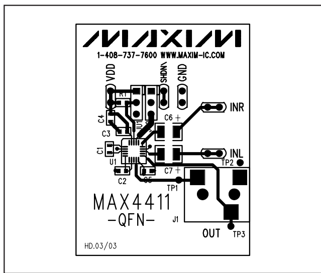
Figure 4. MAX4411 EV Kit Component Placement Guide—Component Side
