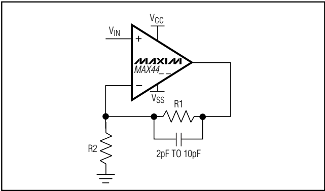
Figure 2. Compensation for Feedback Node Capacitance
