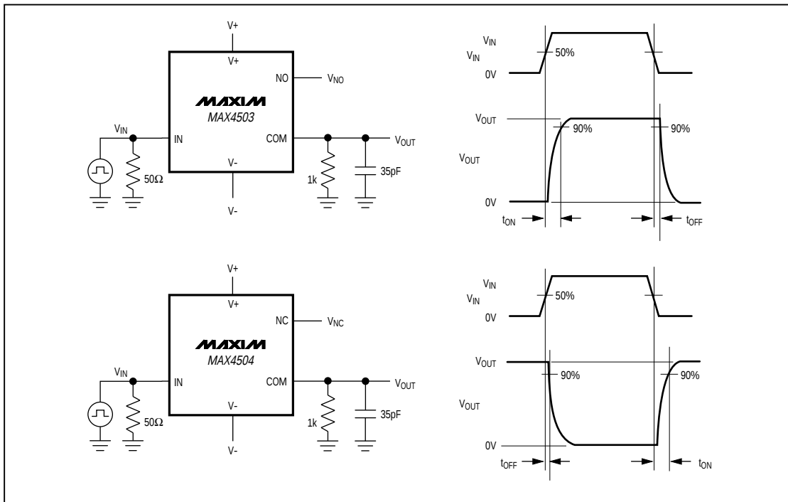
Figure 1. Switching Times
