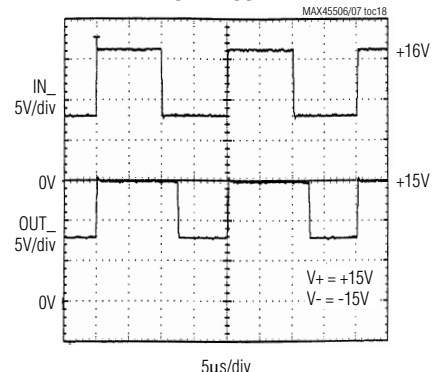
FAULT RECOVERY
