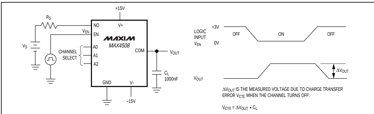
Figure 5. Charge Injection
