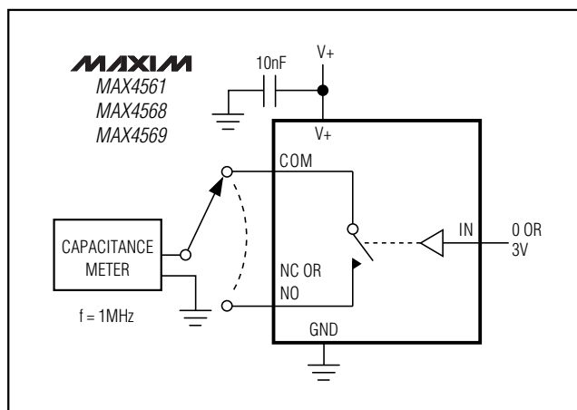
Figure 4. Channel On/Off-Capacitance
