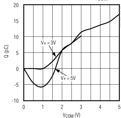
MAX4568/MAX4569 CHARGE INJECTION vs. V_{\text{COM}}
