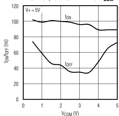
TURN-ON/TURN-OFF TIME vs. V_{\text{COM}}
