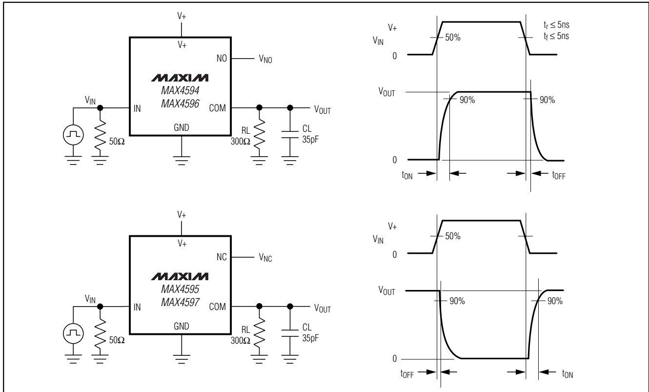
Figure 3. Switching Times
