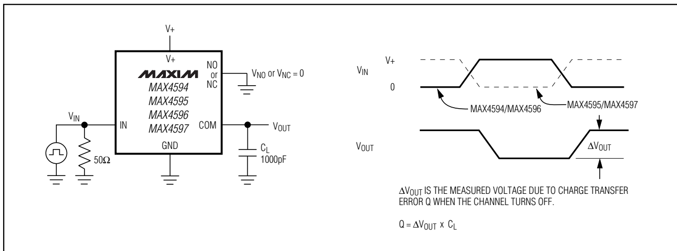
Figure 2. Charge Injection
