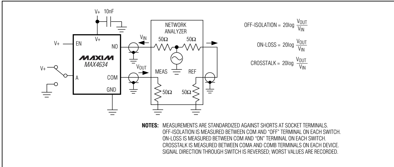
Figure 5. Off-Isolation/On-Channel Bandwidth
