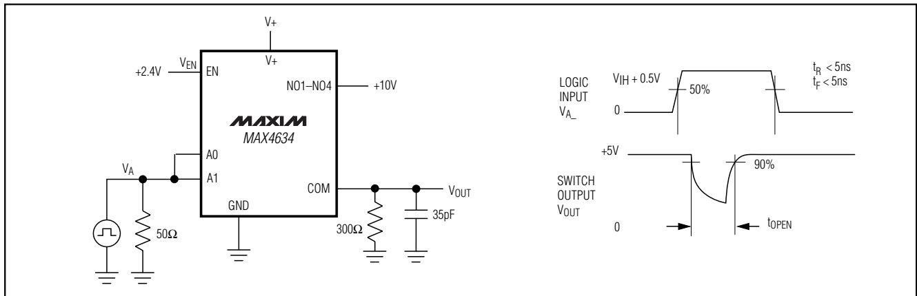
Figure 3. Break-Before-Make Interval
