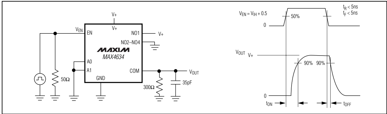
Figure 2. Switching Time
