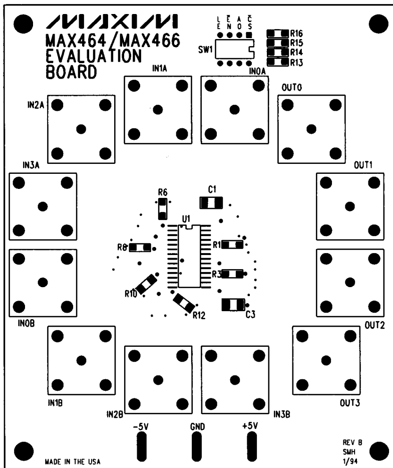
Figure 2. MAX464/MAX466 EV Kit Component Placement Guide—Component Side
