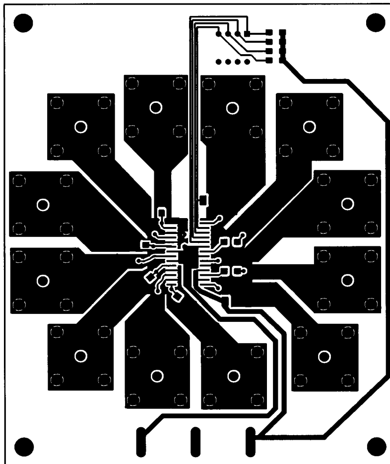
Figure 4. MAX464/MAX466 EV Kit PC Board Layout—Component Side
