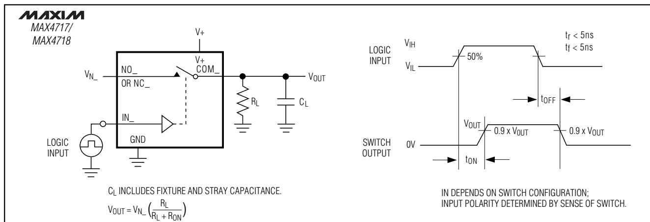
Figure 1. Switching Time
