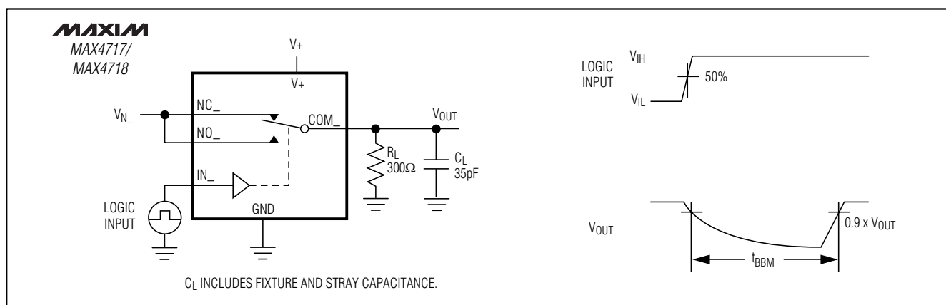
Figure 2. Break-Before-Make Interval
