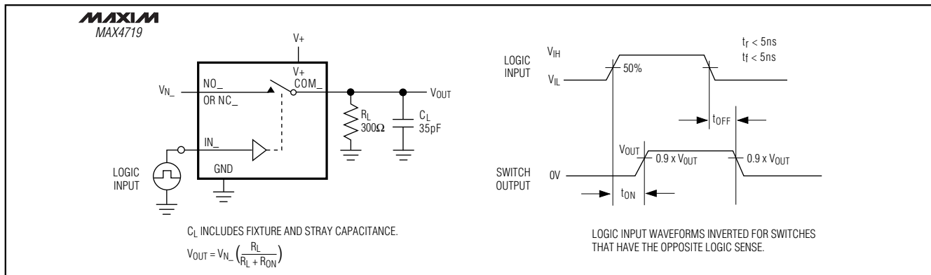
Figure 1. Switching Time
