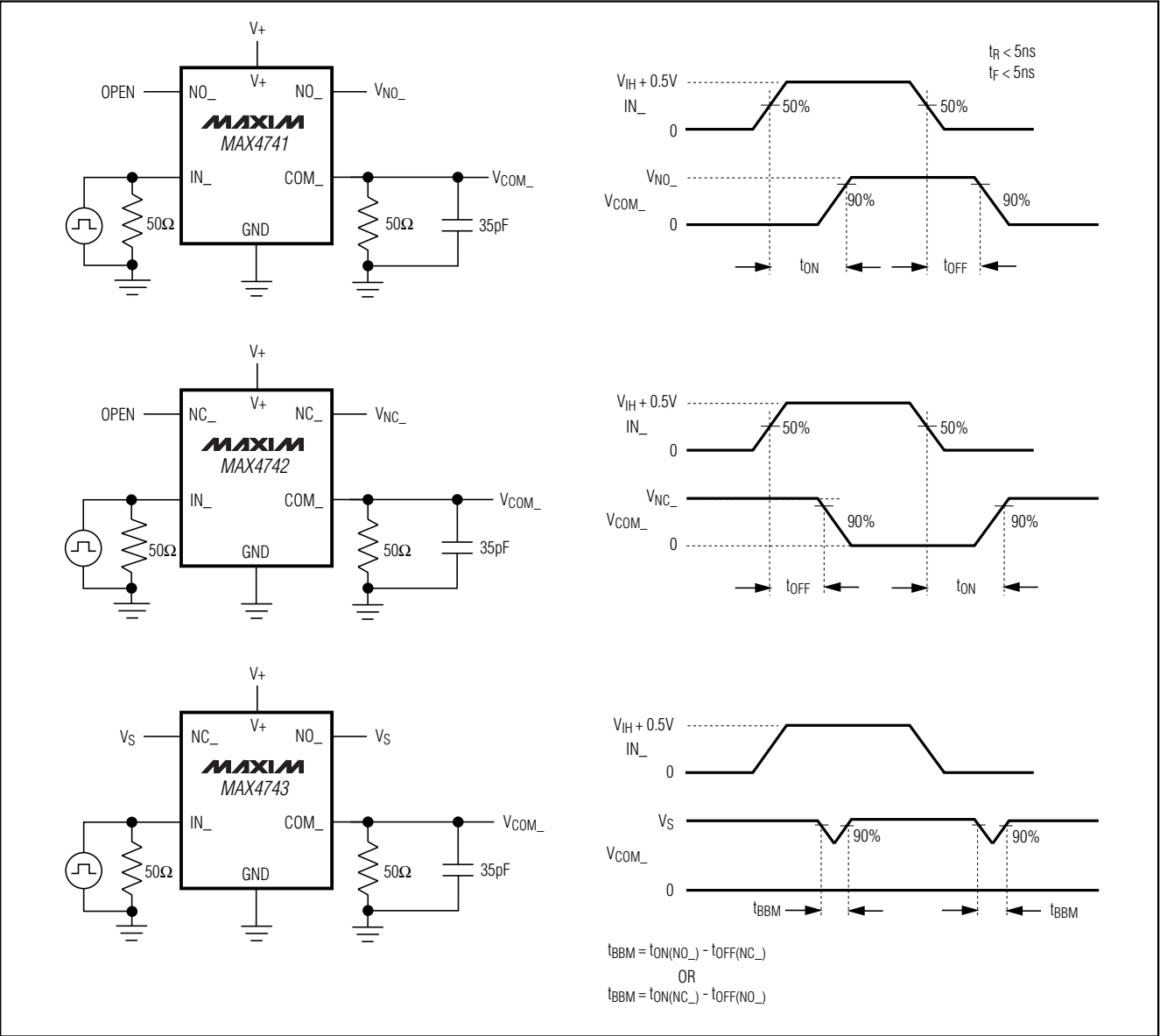
Figure 1. Switching Times
