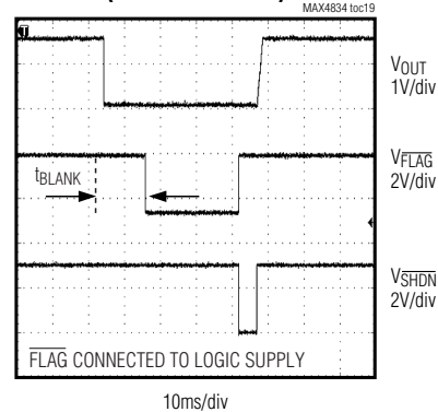
FLAG RESPONSE WHEN OUT IS SHORTED TO GND > BLANKING TIME (SHDN IS TOGGLED)
