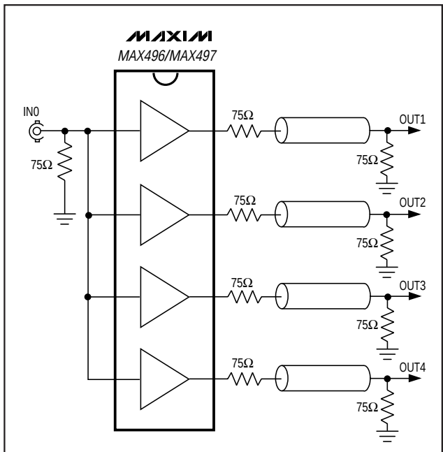
Figure 3. One-to-Four Distribution Amplifier
