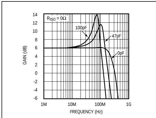
Figure 3a. Small-Signal Gain vs. Frequency and Load Capacitor ( R_L = 100\Omega , R_{ISO} = 0\Omega )
