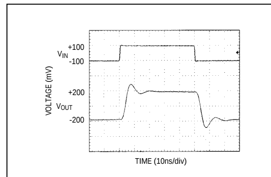
Figure 4b. Small-Signal Pulse Response with C_L = 100\text{pF} and R_{ISO} = 5.1\Omega
