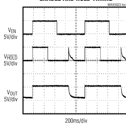
ENABLE AND HOLD TIMING
