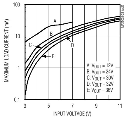
MAX5026 MAXIMUM LOAD CURRENT vs. INPUT VOLTAGE
