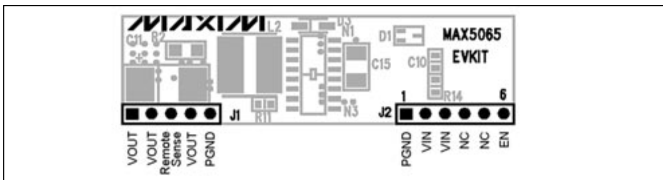
Figure 1. MAX5065 EV Kit Pinout
