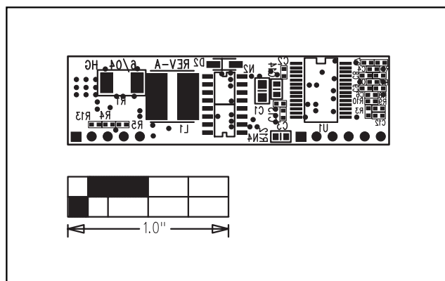
Figure 8. MAX5065 EV Kit Component Placement Guide—Bottom Layer
