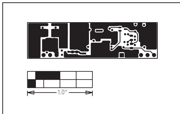
Figure 4. MAX5065 EV Kit PC Board Layout—Top Layer
