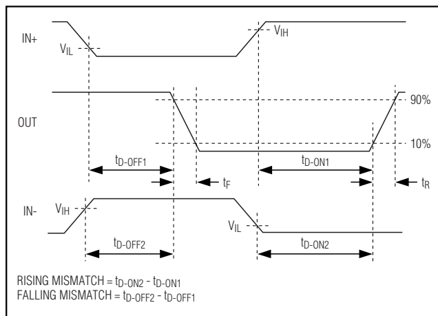
Figure 1. Timing Diagram
