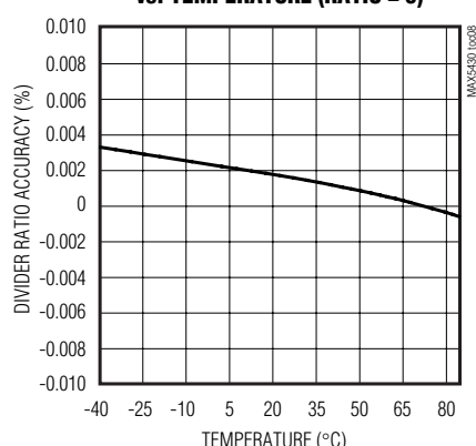
MAX543_B DIVIDER RATIO ACCURACY vs. TEMPERATURE (RATIO = 8)
