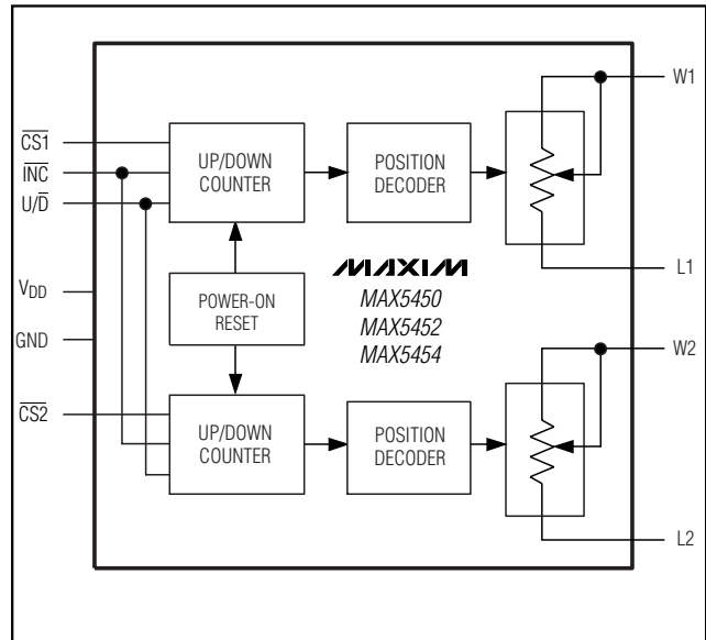
Figure 3. MAX5450/MAX5452/MAX5454 Simplified Functional Diagram
